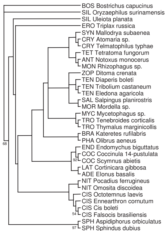
8 R-sample-ML[COI,18S](sct)
