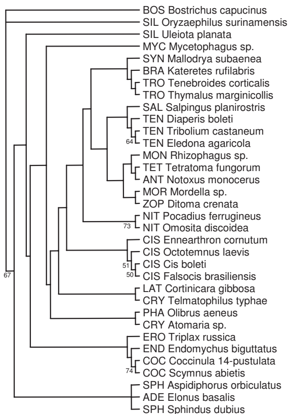
7 R-sample-MPdw[COI,18S](sct)
